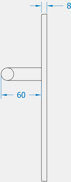
Side Profile
