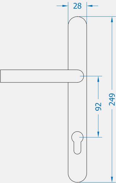
Front Profile
