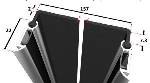
Astro FingerKeeper Industrial TPV Standard Profile (measurements in mm)
