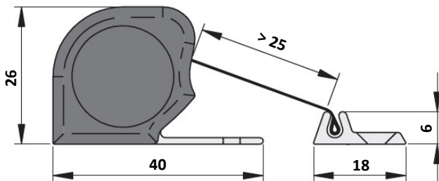
Astro Finger Guard - Washable (measurements in mm)
