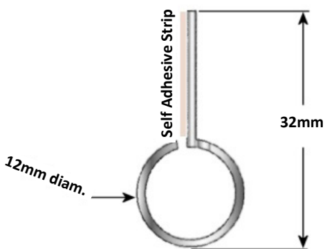
Astro Finger Saver Elite Rear (measurements in mm)
