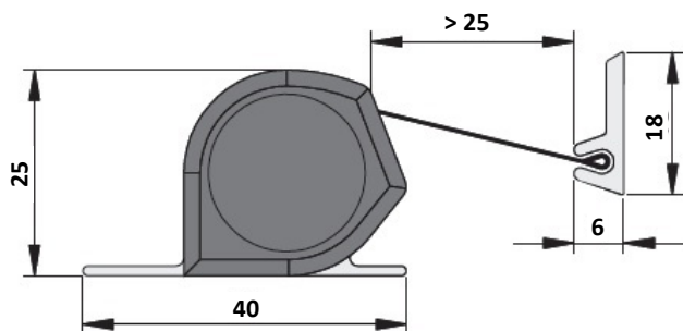
Astro Finger Defender - Glass (measurements in mm)
