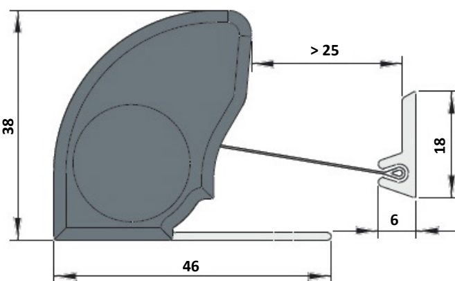
Astro Finger Protecta (measurements in mm)
