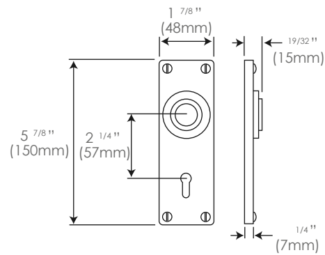
Lock/Keyhole FD175 2 1/4" (57mm lock centres) (un-sprung)
