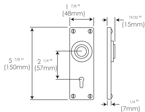
Lock/Keyhole FD192 2 1/4" (57mm lock centres) (un-sprung)
