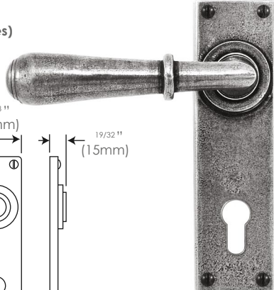
FD061 2 1/4 inches (57mm lock centres) (sprung)
