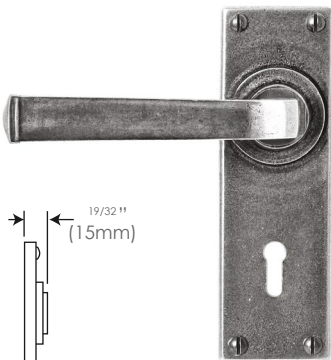
Lock/Keyhole FD013 2 1/4" (57mm lock centres) (sprung)
