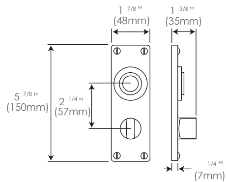
Lock/Keyhole FD175 2 1/4" (57mm lock centres) (un-sprung)
