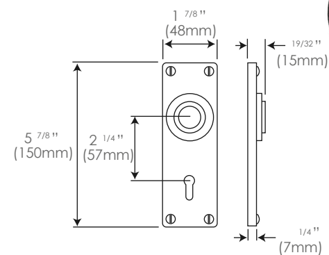
Lock/Keyhole FD040 2 \frac{1}{4}'' (57mm lock centres) (un-sprung)
