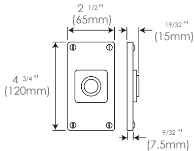
Jesmond Bathroom FD169 Oak FD170 American Black Walnut (sprung)
