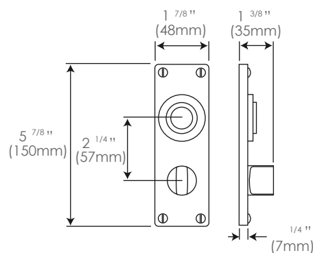
Lock/Keyhole FD192 2 1/4" (57mm lock centres) (un-sprung)
