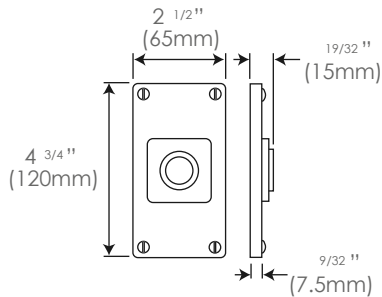
Jesmond Bathroom FD196 (un-sprung)
