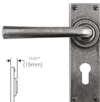
Euro Lock/Keyhole FD303E4 1 7/8" (47.5mm lock centres) (sprung)
