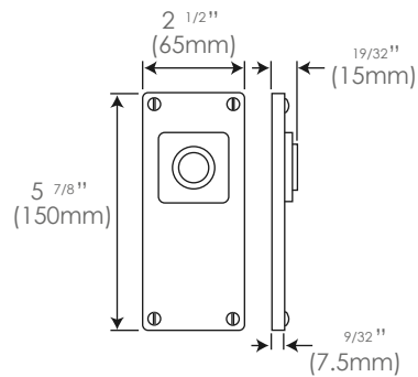
Jesmond Lock/Keyhole FD179 2 1/4" (57mm lock centres) (un-sprung)
