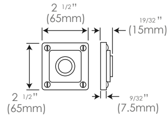
Jesmond Long Latchplate FD177 (un-sprung)
