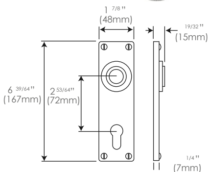
FD065E7 2 53/64" (72mm lock centres) (sprung)
