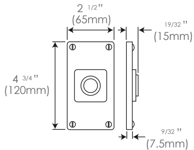
Jesmond Bathroom FD081 (un-sprung)
