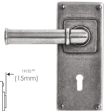
Jesmond Lock/Keyhole FD188 2 1/4" (57mm lock centres) (sprung)
