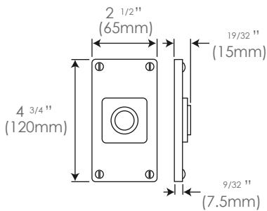
Jesmond Bathroom FD069 (sprung)
