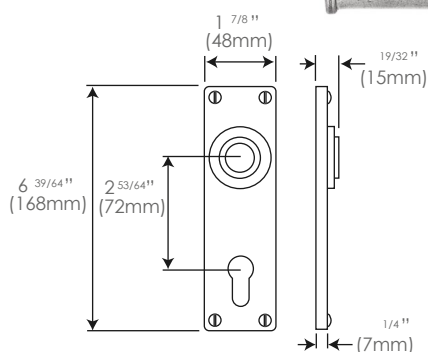
FD183E7 2 53/64 inches (72mm lock centres) (sprung)
