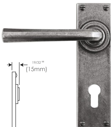
Euro Lock/Keyhole FD303E7 2 53/64" (72mm lock centres) (sprung)
