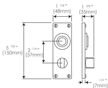
Lock/Keyhole FD303 2 1/4" (57mm lock centres) (sprung)
