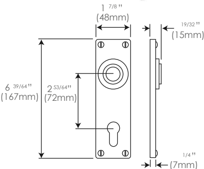
Euro Lock/Keyhole FD013E7 2 53/64" (72mm lock centres) (sprung)
