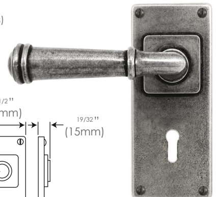
Jesmond Lock/Keyhole FD070 2 1/4" (57mm lock centres) (sprung)
