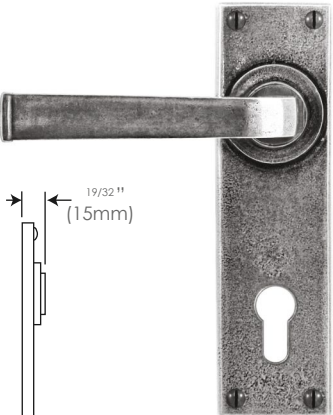
Euro Lock/Keyhole FD013E7 2 53/64" (72mm lock centres) (sprung)
