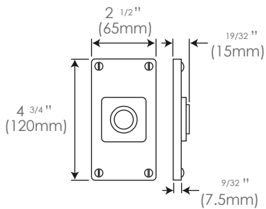
Jesmond Bathroom FD187 (sprung)
