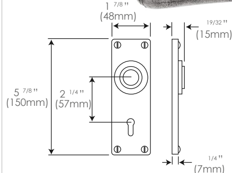
FD061 2 1/4 inches (57mm lock centres) (sprung)
