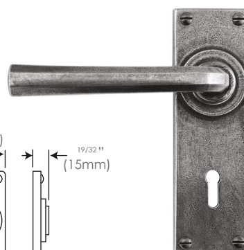
Lock/Keyhole FD303 2 1/4" (57mm lock centres) (sprung)
