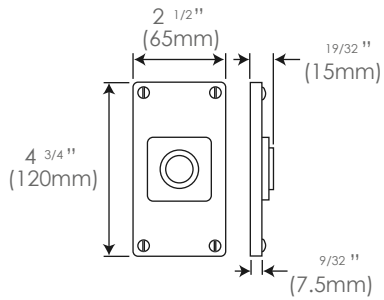
Jesmond Bathroom FD085 (un-sprung)
