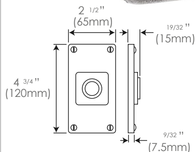
Jesmond Bathroom FD089 (sprung)
