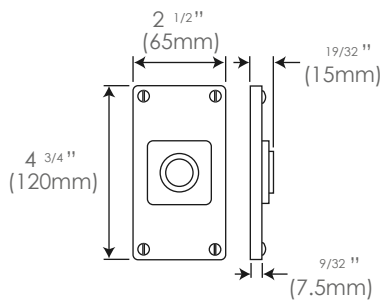
Jesmond Bathroom FD178 (un-sprung)
