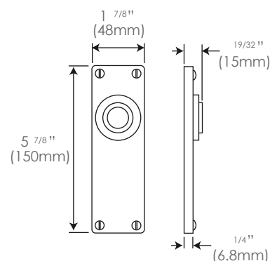
Bathroom FD035 (un-sprung)
