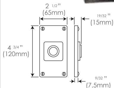
Jesmond Bathroom FD307 (sprung)
