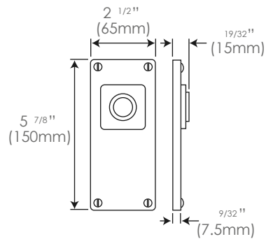
Jesmond Lock/Keyhole FD197 2 1/4" (57mm lock centres) (un-sprung)
