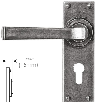
Euro Lock/Keyhole FD013E4 1 7/8" (47.5mm lock centres) (sprung)
