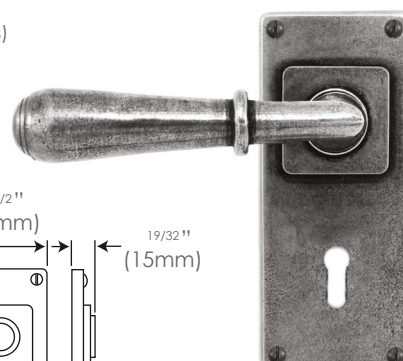
Jesmond Lock/Keyhole FD090 2 1/4" (57mm lock centres) (sprung)
