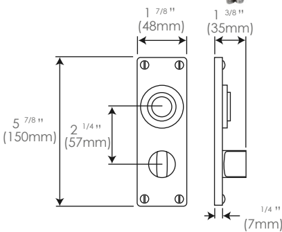
Lock/Keyhole FD005 2 1/4" (57mm lock centres) (sprung)
