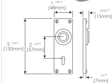
FD065 2 1/4" (57mm lock centres) (sprung)
