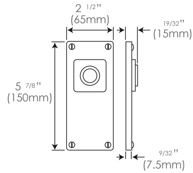
Jesmond Lock/Keyhole FD086 2 1/4" (57mm lock centres) (un-sprung)
