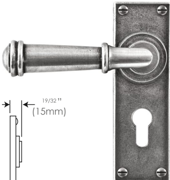
Euro Lock/Keyhole FD005E4 1 7/8" (47.5mm lock centres) (sprung)
