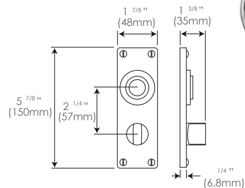
Lock/Keyhole FD036 2 1/4" (57mm lock centres) (un-sprung)
