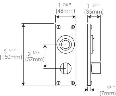
Lock/Keyhole FD013 2 1/4" (57mm lock centres) (sprung)
