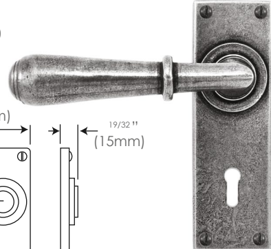
FD061 2 1/4 inches (57mm lock centres) (sprung)
