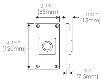
Jesmond Bathroom FD073 (sprung)
