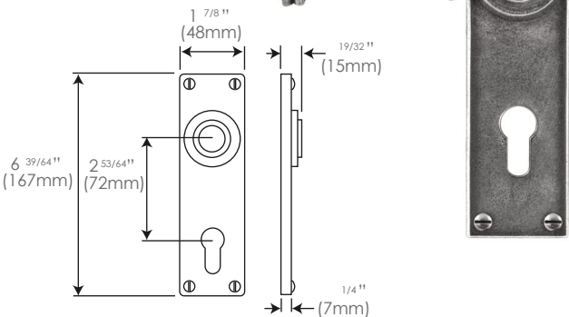
Euro Lock/Keyhole FD005E7 2 53/64" (72mm lock centres) (sprung)
