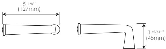
Euro Lock/Keyhole FD013E4 1 7/8" (47.5mm lock centres) (sprung)
