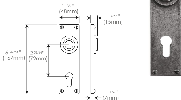
Euro Lock/Keyhole FD303E7 2 53/64" (72mm lock centres) (sprung)
