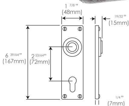
FD061E7 2 53/64 inches (72mm lock centres) (sprung)
