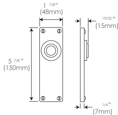
Bathroom FD174 (un-sprung)
