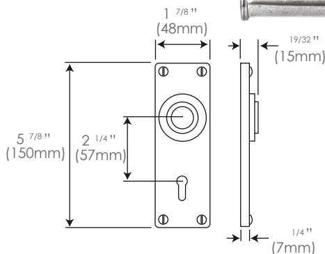
FD183 2 1/4 inches (57mm lock centres) (sprung)
