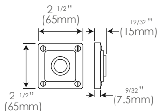
Jesmond Long Latchplate FD115 (sprung)
