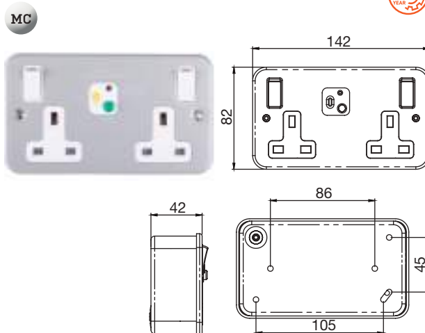
MC5023 RCD double socket
