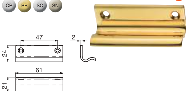
AQ50 Sash window lift
