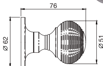
M48 Ball mortice knob Solid half sprung
