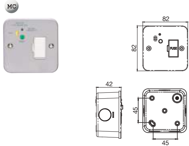
MC5033 RCD socket fuse
