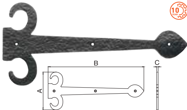
LF5121 LF5122 LF5123 Sword hinge front
