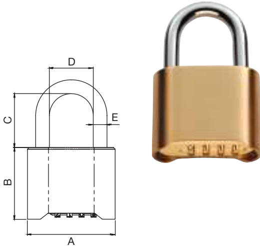
Heavy duty combination padlock Bottom wheel
