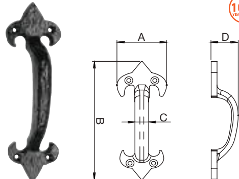
LF5574A LF5574B LF5574C Pull handle
