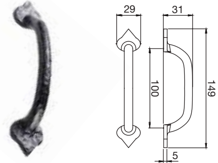
FTD1068B Hammered Fleur de Lys handle
