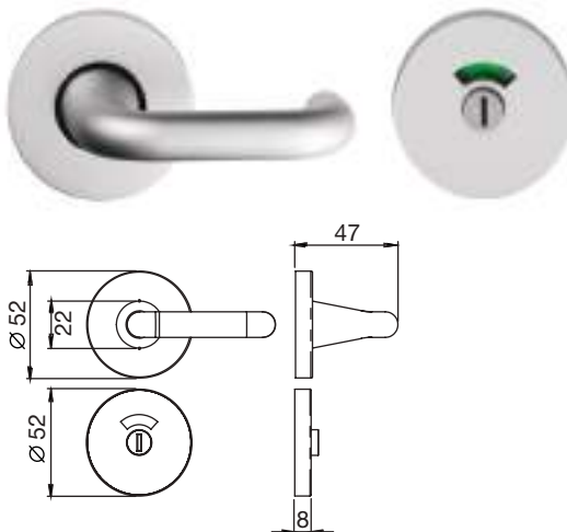
EST9025 Thumbturn & release with indicator
