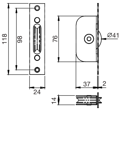
AQ93 Sash window axle pulley square forend with brass wheel
