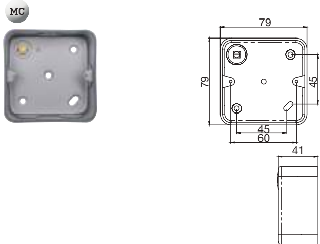
MC8014 Single back box
