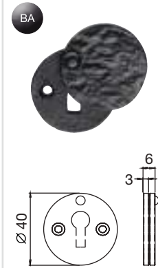
LF5546 Lock covered escutcheon
