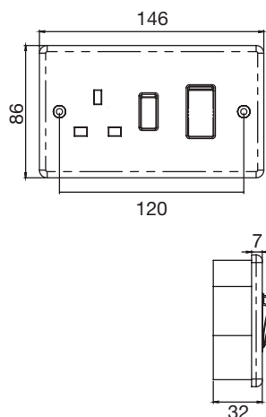
PL3310 45 DP switch and 13 Amp switched socket
