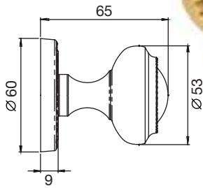
M35RS Small Mushroom rim knob Unsprung
