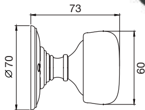
DK35C Plain knob concealed fix Unsprung
