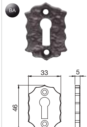
LF5531 Lock floral escutcheon
