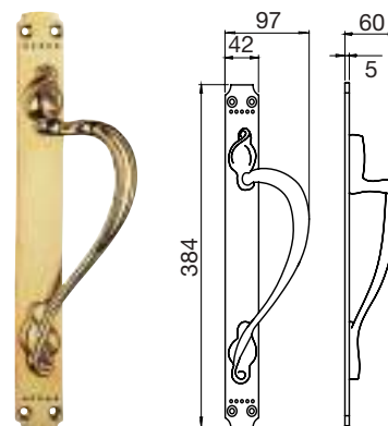
PF109AL Left hand
