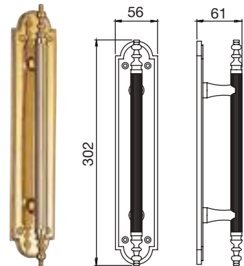
PF109AR Laurin pull handle Right hand
