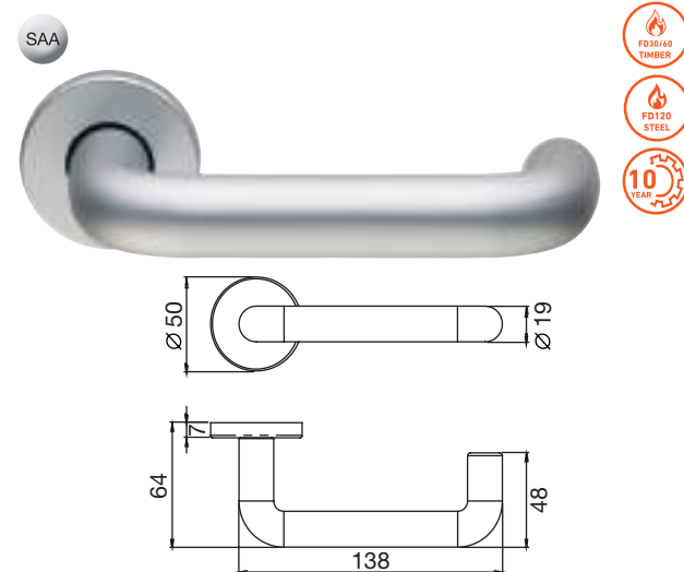
LRS4001 Safety lever on sprung rose bar 19mm diameter
