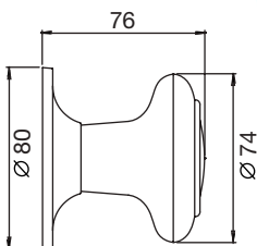
M61 Round centre door knob
