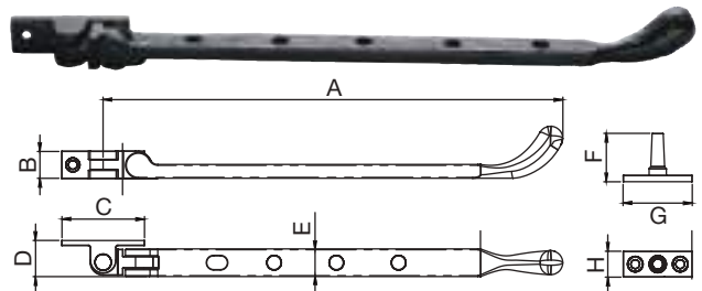
LF5544B LF5544C Bulb end casement stay
