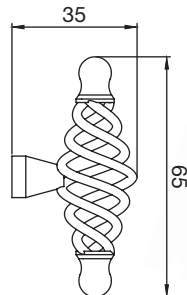
FTD1230B Steel cage oval knob
