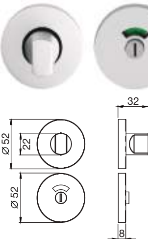
EST9005 Thumbturn & release with indicator
