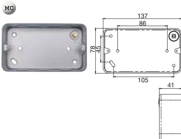
MC8024 2 Gang metal clad box with terminal
