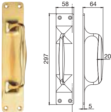
PF103ER Engraved large pull handle Right hand
