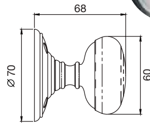
DK34ICFB Porcelain knob face fix Unsprung
