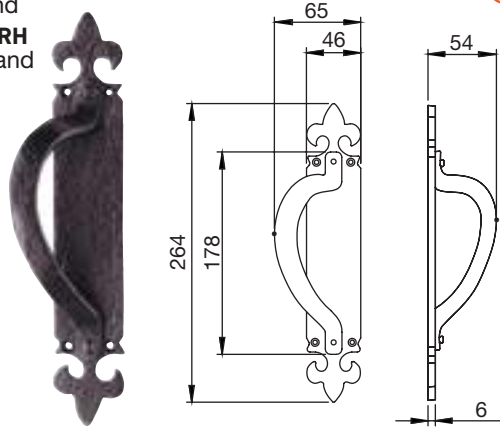
LF5575A LF5575B Hotbed handle
