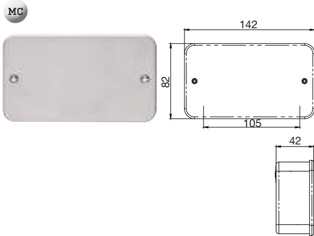
MC2B Double blank plate
