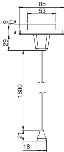
PL3331 45 Amp Pull cord ceiling switch with neon
