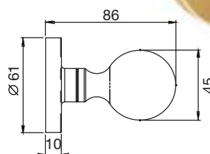
M35C Mushroom mortice knob concealed fix Unsprung
