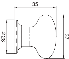
FTD1230B Steel cage oval knob
