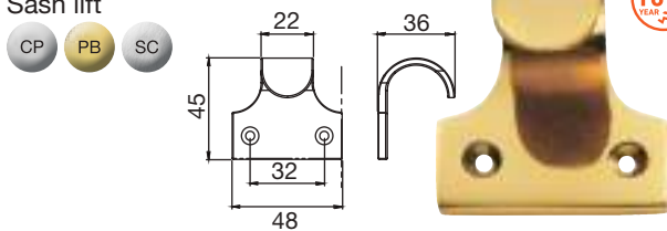
AQ50 Sash window lift
