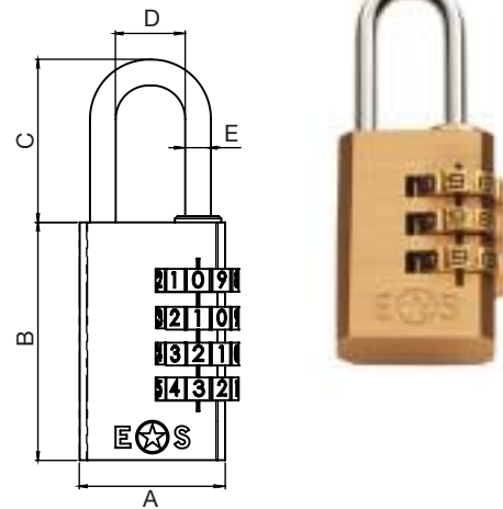
Combination padlock Side wheel
