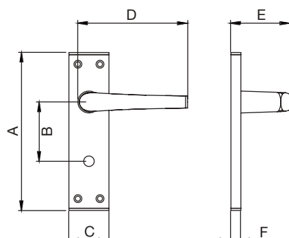
SAA61 Short plate latch
