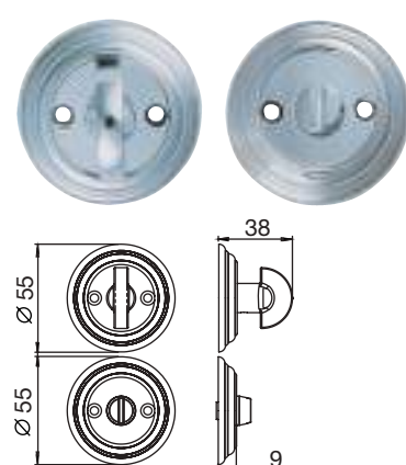
DK12 Large thumbturn & release
