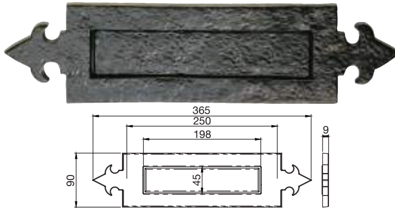
LF5524 Traditional letter plate
