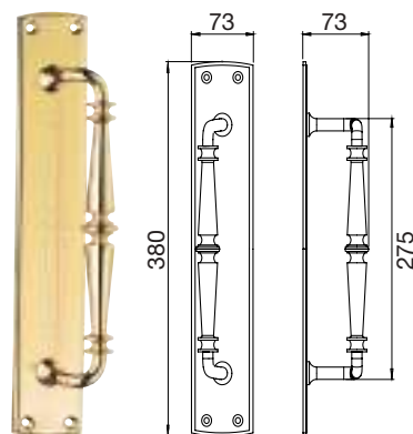
PF105E Engraved large push plate
