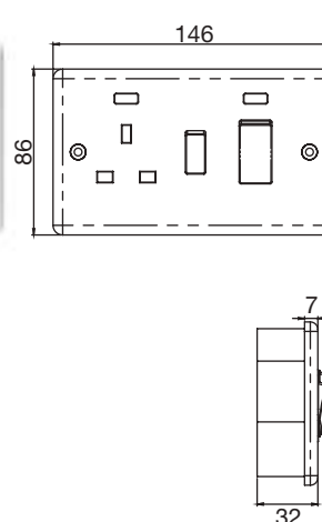
PL3311 45 DP switch and 13 Amp switched socket with neon
