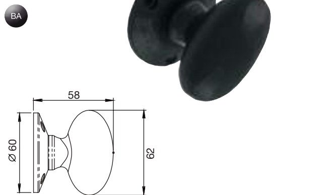
LF5595 Oval mortice knob Half-sprung
