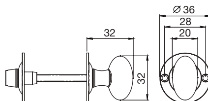
AA33MB Oval thumbturn Spline spindle to operate rack bolt
