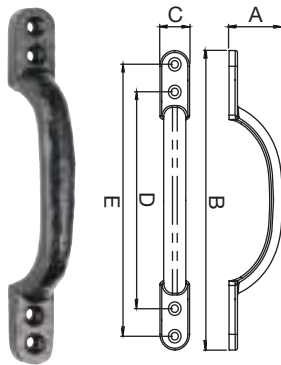
LF5575A LF5575B Hotbed handle
