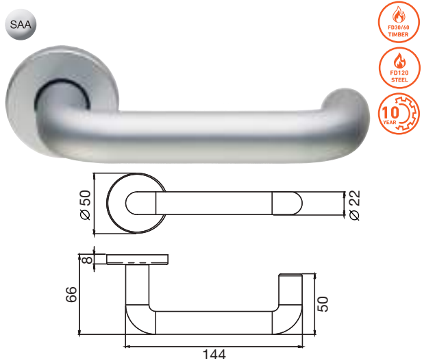
LRS4000 Safety lever on sprung rose bar 22mm diameter
