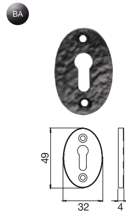
LF5533 Lock shield covered escutcheon
