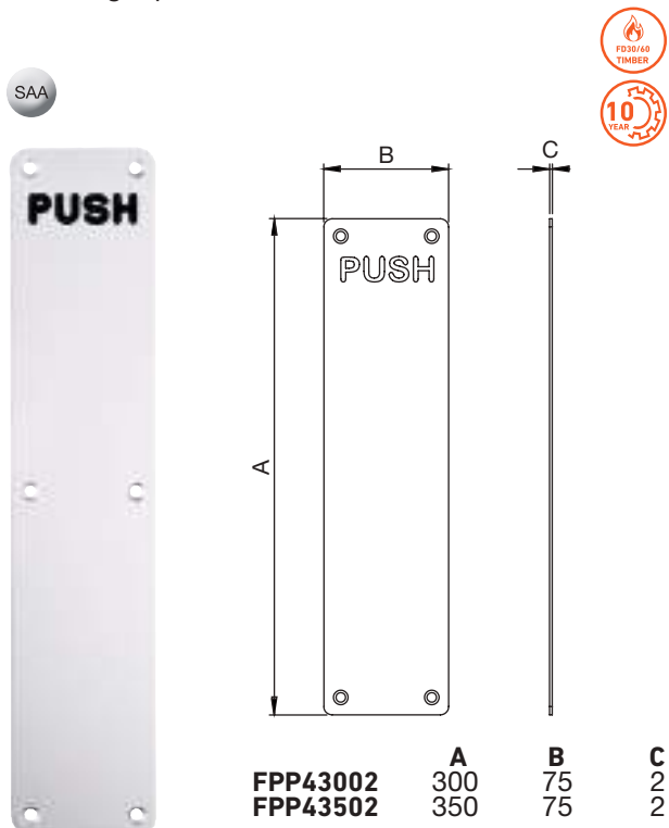
Push finger plate
