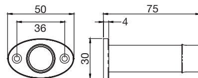
LF5547 Ring handle gate latch
