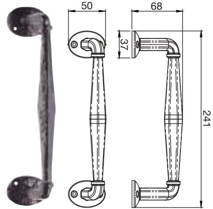
LF5266 Offset pull handle on rose
