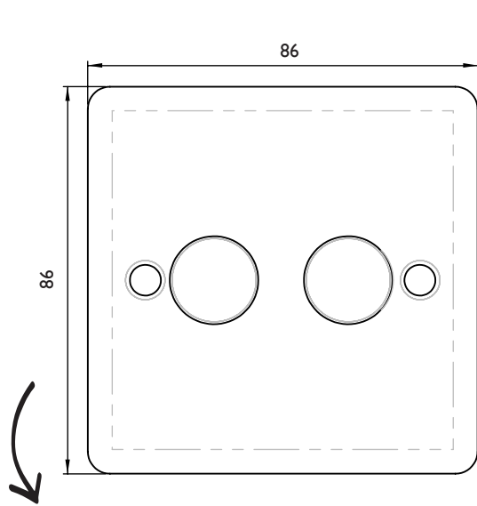
Front profile 2 Gang Dimmer
