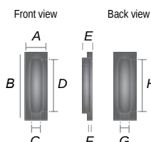
C1850 105 Flush Pull Handle
