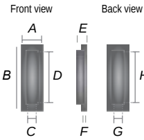
C1865 [Design Reg: 6202496] Reeded Rectangular Flush Note: The recess measurement required to fit this item is taken from the back Sold and supplied in singles
