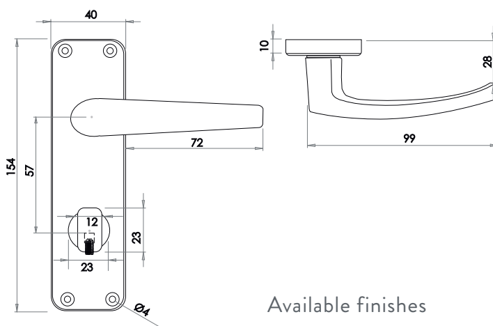
Bathroom Long Plate
