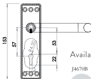
Lockset - Standard Keyway
